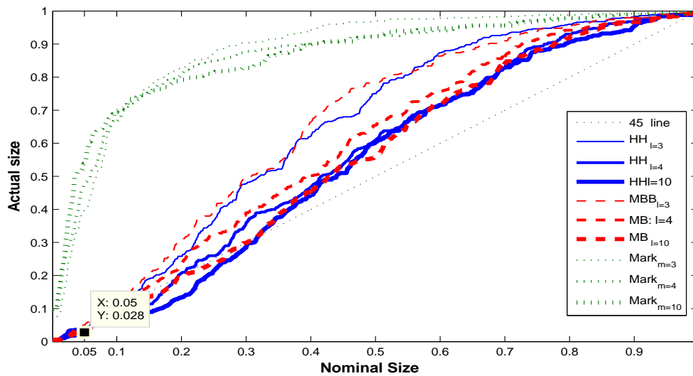
Figure 13: Fast Bootstrap RP1 plot for J-test under the Null Model NRF1 . The sample size is T = 120 , block length, l equal to markov lag m , and instruments lag = 1
