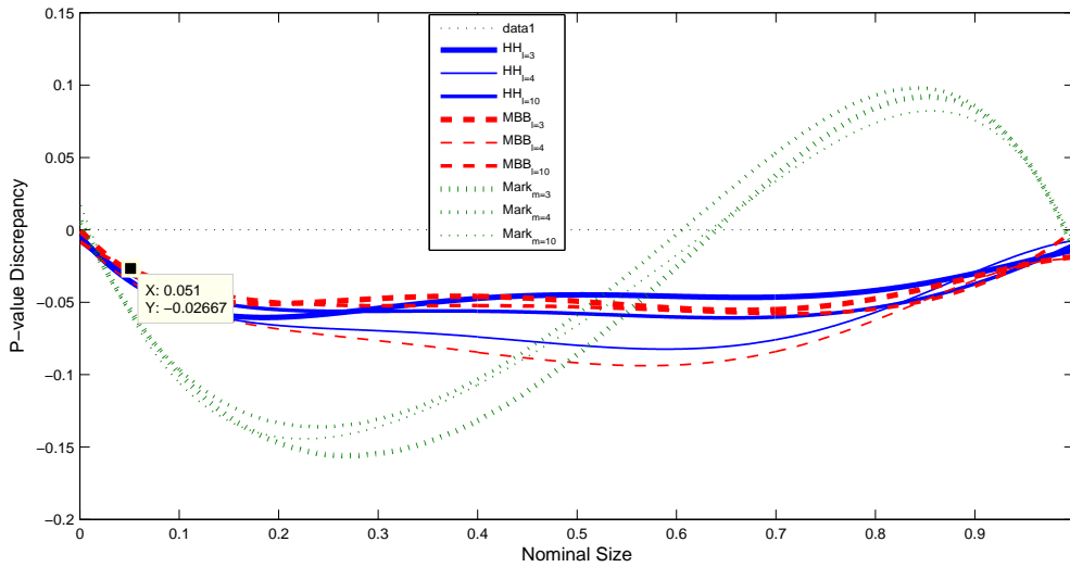
Figure 7: Smoothed Bootstrap P-value discrepancy ERP1 plot for J-test under the Null Model FR1 . The sample size is T = 120 , block length, l equal to markov lag m , and instruments lag = 1
