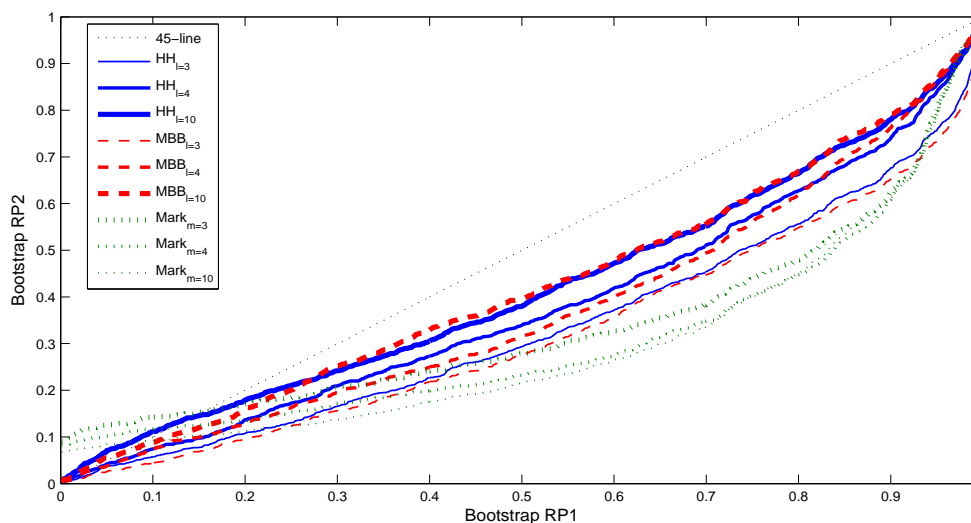
Figure 10: Fast Bootstrap RP1 and RP2 plot for J-test under the Null Model FR1 . The sample size is T = 120 , block length, l equal to markov lag m , and instruments lag = 4
