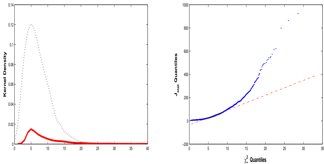
Figure 12: The Empirical Distribution of J-test under the Null Model FR1 and the Quantile plot against the Asymptotic \chi^2 distribution. The sample size is T = 120 , and instruments lag = 4 .
