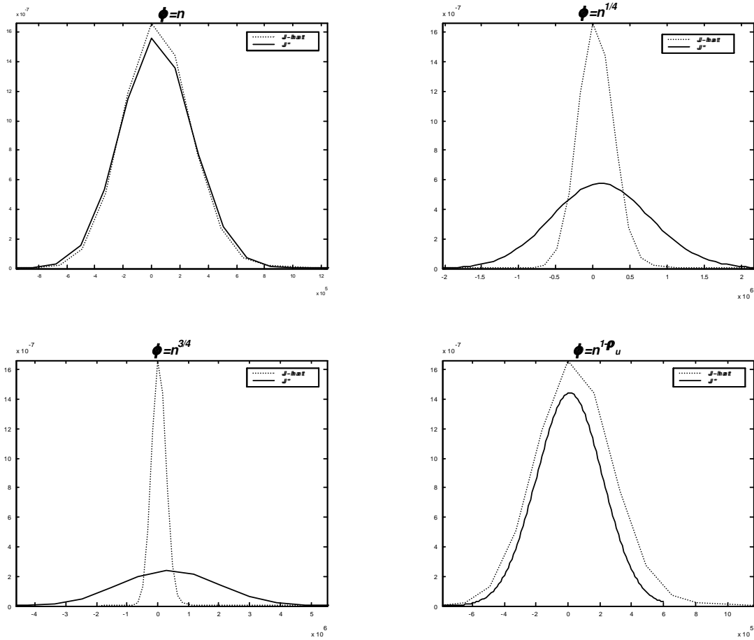
Figure 3: Plot of distribution of a Bootstrap (solid) J – test, J^* statistic and the Empirical distribution of the test (dotted), \hat{J} , case lag = 4 and correlation parameter \rho_\mu = 0.25 .
