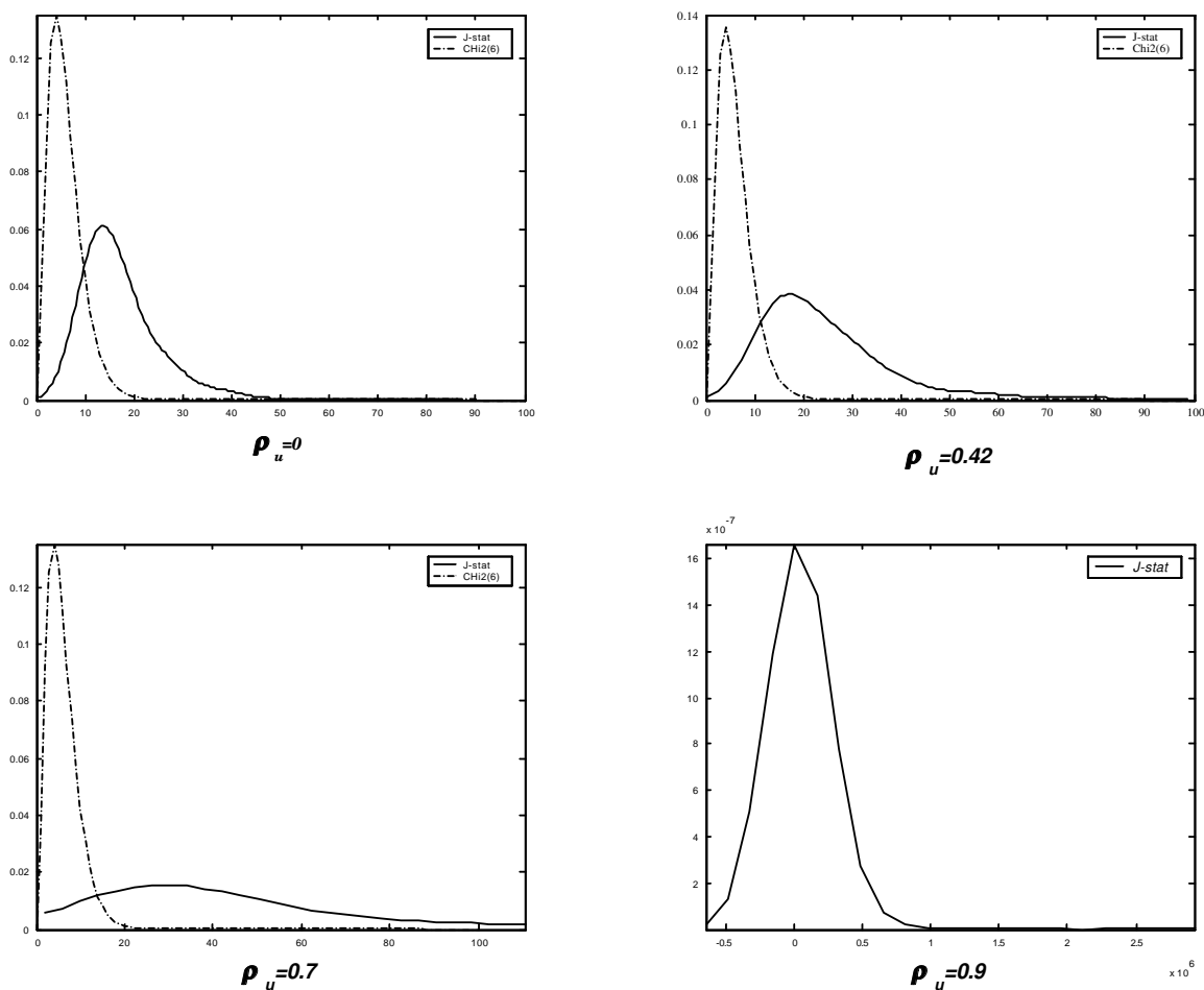
Figure 1: The Sampling Distribution of the J - test, \hat{J} , statistic (solid line), case lag = 1 and correlation parameter \rho_\mu against the asymptotic \chi_6^2 distribution (dotted line).
