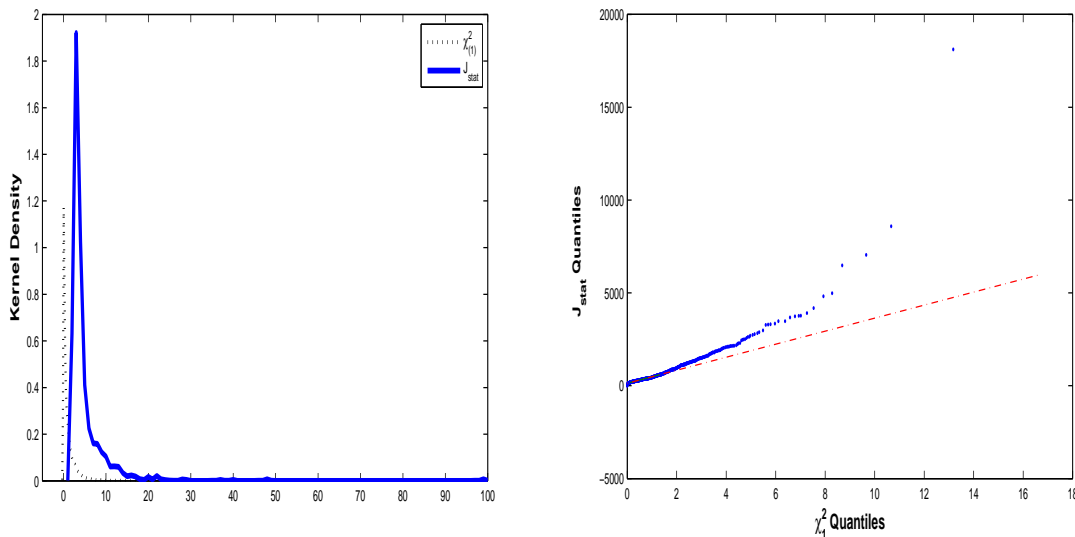
Figure 16: The Empirical Distribution of J-test under the Null Model NRF1 and the Quantile plot against the Asymptotic \chi^2 distribution. The sample size is T = 120 , and instruments lag = 1 .
