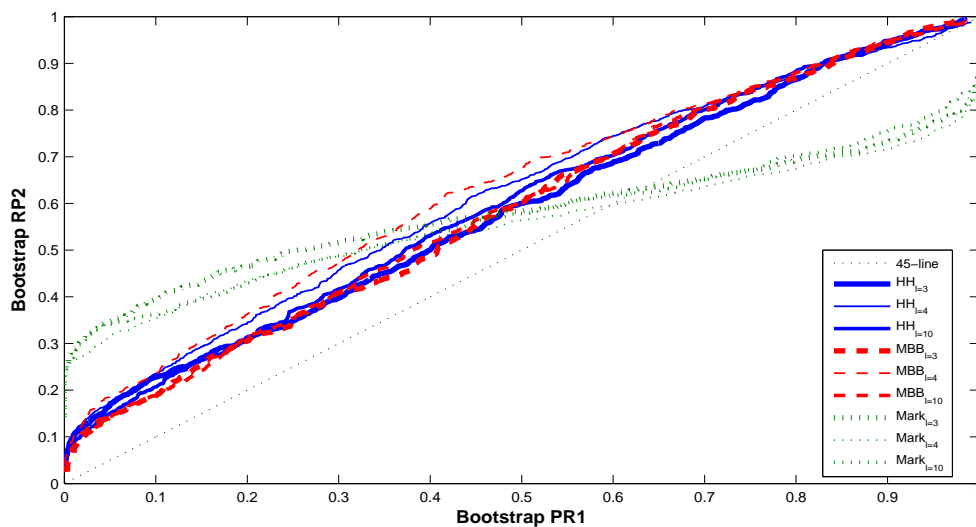
Figure 6: Fast Bootstrap RP1 and RP2 plot for J-test under the Null Model FR1 . The sample size is T = 120 , block length, l equal to markov lag m , and instruments lag = 1
