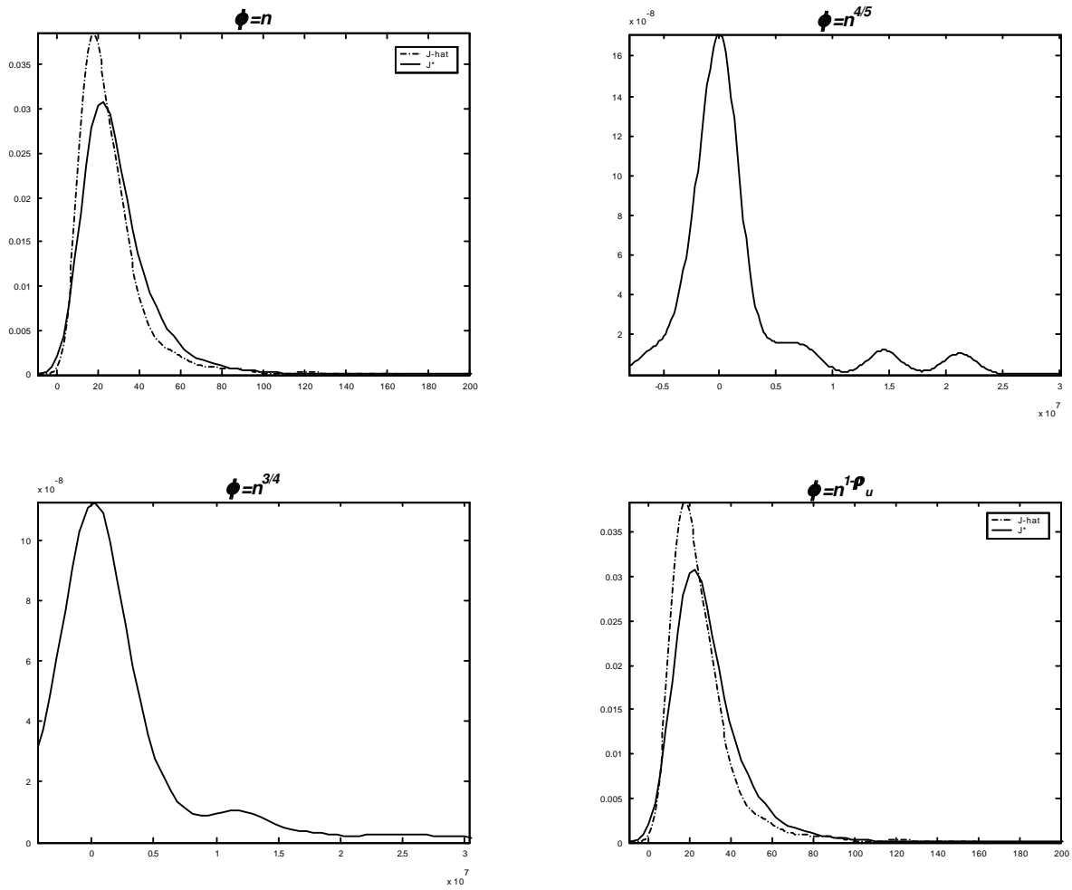
Figure 2: Distribution of the Bootstrap J – statistic (solid line), case lag = 1 and correlation parameter \rho_\mu = 0 for different values of \phi
