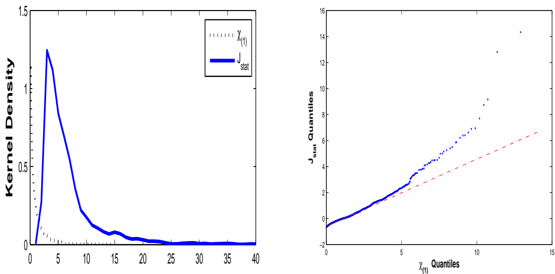
Figure 8: The Empirical Distribution of J-test under the Null Model FR1 and the Quantile plot against the Asymptotic \chi^2 distribution. The sample size is T = 120 , and instruments lag = 1 .
