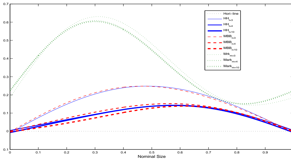
Figure 15: Smoothed Bootstrap P-value discrepancy ERP1 plot for J-test under the Null Model NRF1 . The sample size is T = 120 , block length, l equal to markov lag m , and instruments lag = 1
