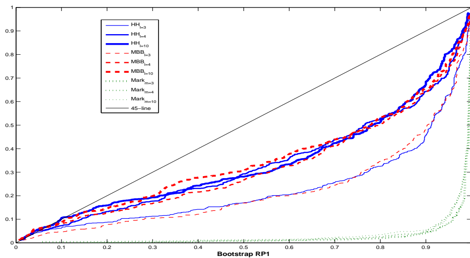
Figure 14: Fast Bootstrap RP1 and RP2 plot for J-test under the Null Model NRF1 . The sample size is T = 120 , block length, l equal to markov lag m , and instruments lag = 1
