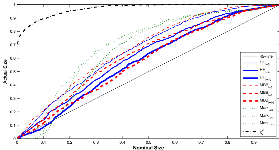
Figure 9: Fast Bootstrap RP1 plot for J-test under the Null Model FR1 . The sample size is T = 120 , block length, l equal to markov lag m , and instruments lag = 4
