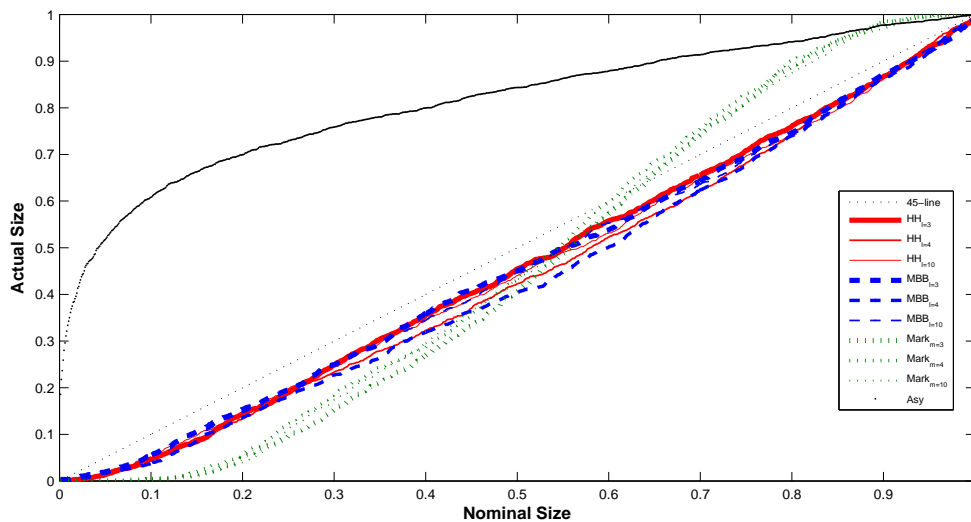
Figure 5: Fast Bootstrap RP1 plot for J-test under the Null Model FR1 . The sample size is T = 120 , block length, l equal to markov lag m , and instruments lag = 1
